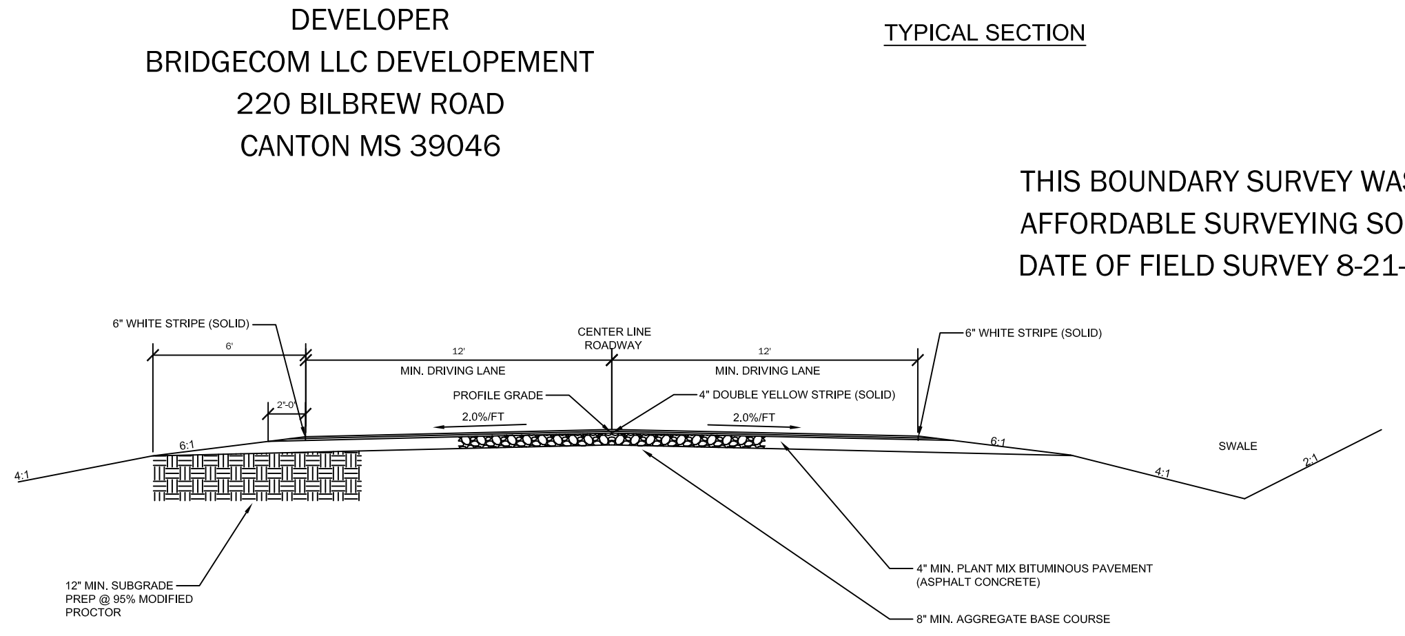
TYPICAL SECTION
